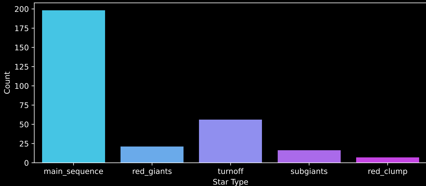
GALAH DR4 Field: [7046] Count plot of Star Type
