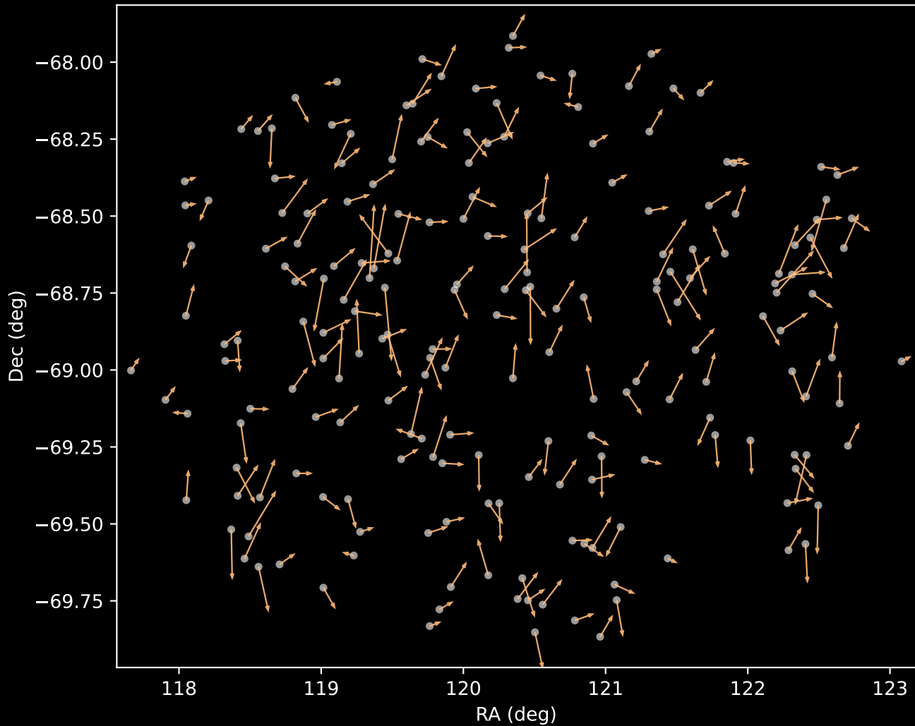
GALAH DR4 Cluster 3 Proper Motion Vectors (n=201)
