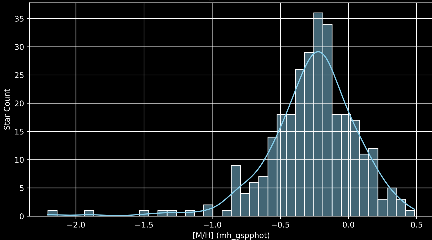
GALAH DR4 Field: [7046] [M/H] (mh_gspphot) (n= 298)
