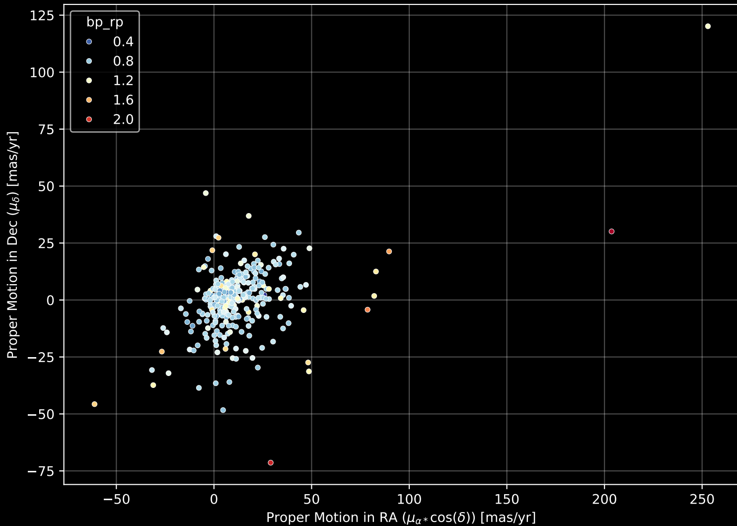
GALAH DR4 Field: [7046] Proper Motion Diagram (n= 298)
