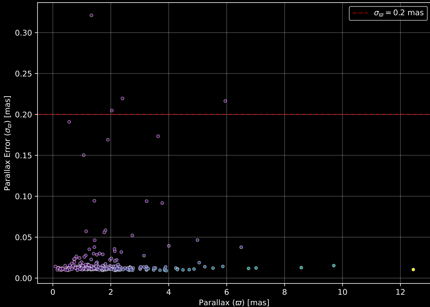
GALAH DR4 Field: [7046] Parallax Quality (n= 298)
