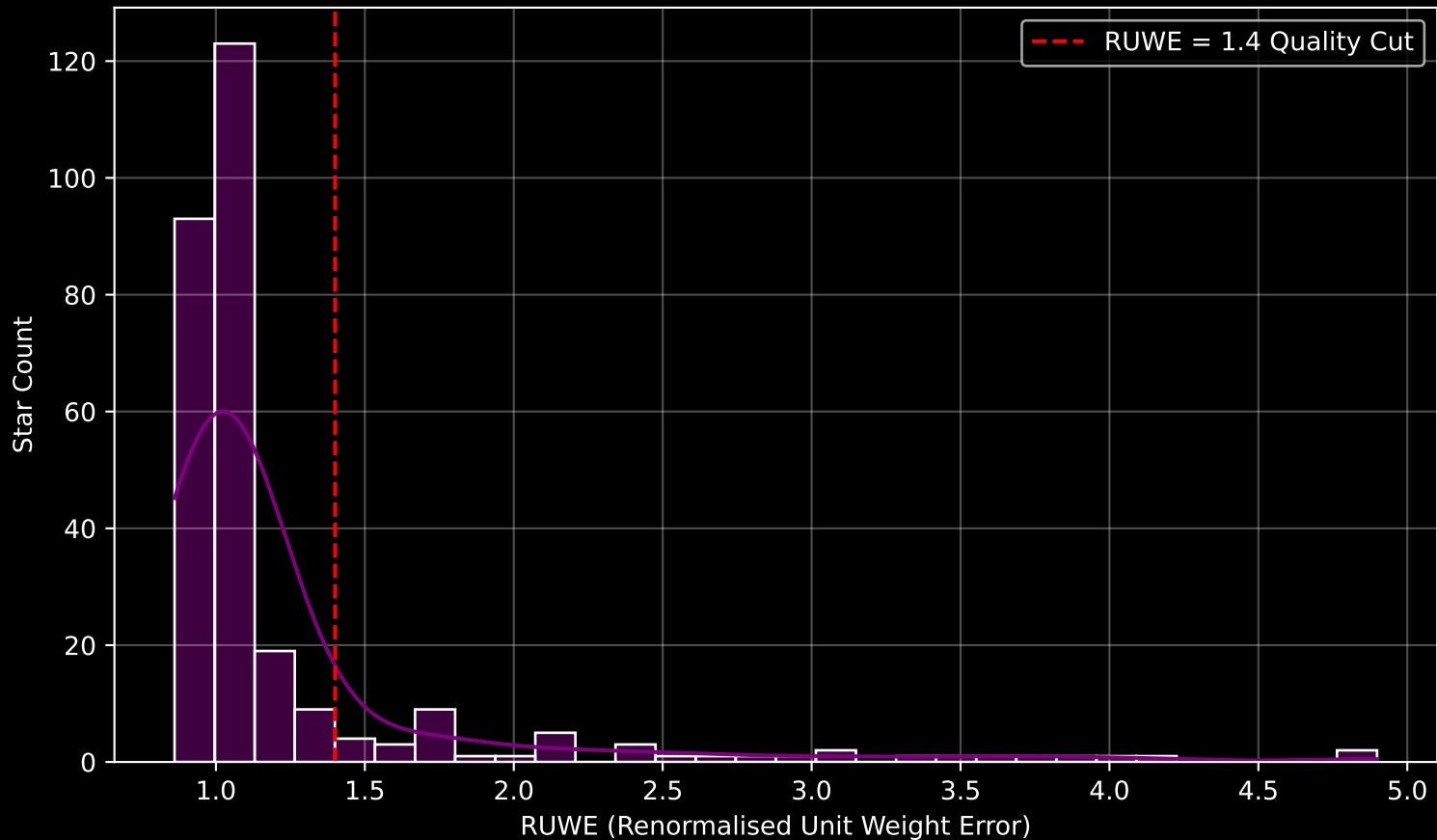
GALAH DR4 Field [7046] RUWE Distribution (n= 285)
